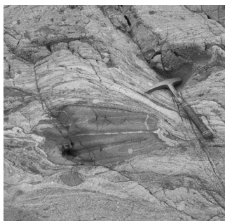
Migmatites of the Southern Flank of the Velay Massif, Pont de Bayzan, Ardèche River.
